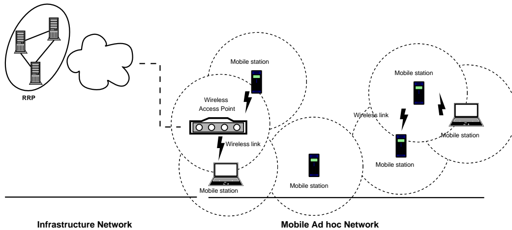
Figure 2: Network architecture
