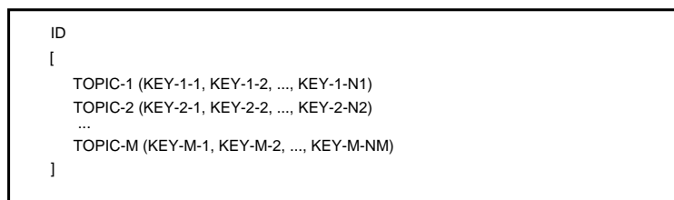
Figure 1: QUERY announcement message format
