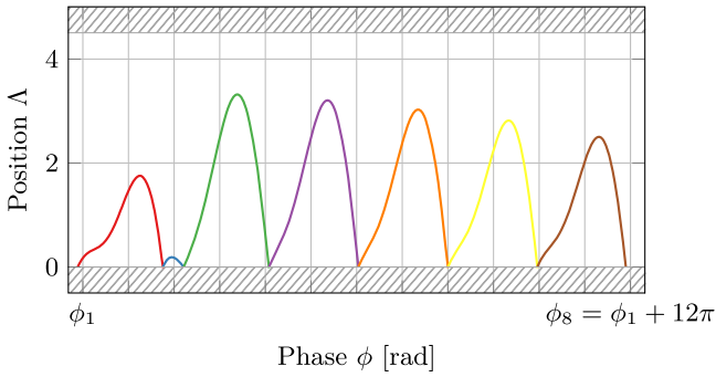
FIG. 6. Trajectory of the electrons in the SS ( \Pi = 12\pi , n_\phi = 7 ). V_d = 33.0 V, \phi_1 = 2.650 rad, and E_0 = 6.03 kV cm ^{-1} .
