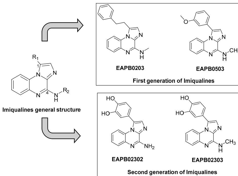
Scheme 1. General and lead compounds structures of the imiqualines.
