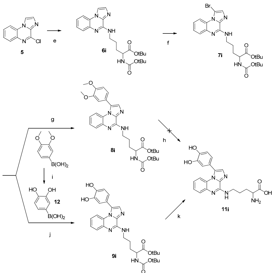
Scheme 3. Synthesis of the ornithine-containing imidazo[1,2- a ]quinoxaline derivative grafted by the side chain. Reagents and Conditions: (e) Boc-Orn-OtBu, HCl, DIEA, DMF, MW (150 °C, 30–60 min); (f) NBS, \text{CHCl}_3 , reflux, 2 h; (g) 3,4-dimethoxyphenylboronic acid, \text{Pd}(\text{PPh}_3)_4 , \text{Na}_2\text{CO}_3 , DME, MW (140 °C, 20 min); (h) \text{BBr}_3 , \text{CH}_2\text{Cl}_2 , RT, 1 h–3 h; (i) \text{BBr}_3 , \text{CH}_2\text{Cl}_2 , RT, 1 h; (j) 3,4-dihydroxyphenylboronic acid 12 , \text{Pd}(\text{PPh}_3)_4 , \text{Na}_2\text{CO}_3 , DME, MW (140 °C, 20 min); (k) TFA/ \text{CH}_2\text{Cl}_2 (1/1, v/v ), RT, 1–2 h.
