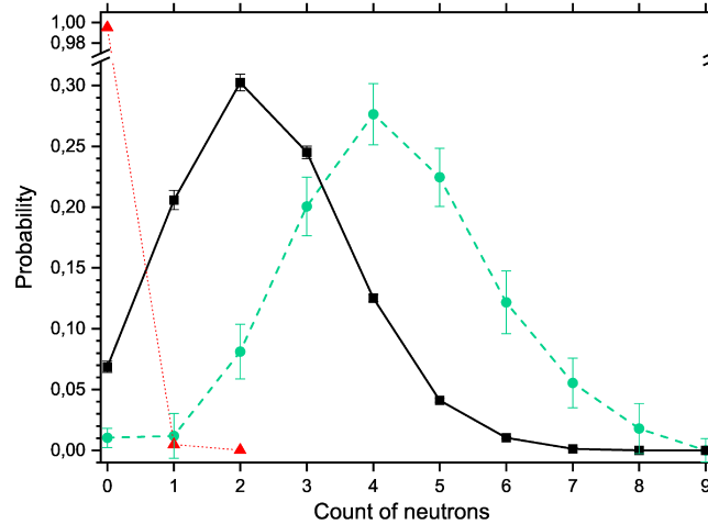
Fig. 2. Measured (squares) and restored (circles) prompt neutron multiplicity distributions of ^{252}\text{No} and background neutron spectra (triangles). Lines that connect the points have been added for clarity.
