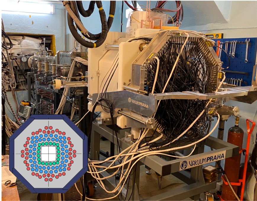
Fig. 1. Photograph of the SFiNx system. A schematic front view of the assembly is shown in the inset image.
