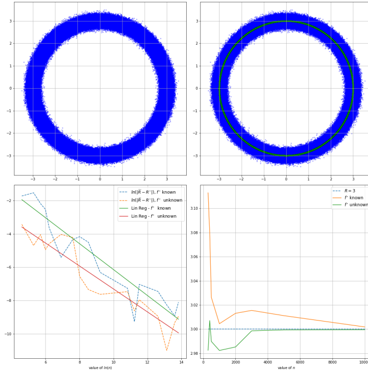
Figure 1: U \sim \text{Unif}(0, 1) , \varepsilon \sim \mathcal{N}(0, (0.12)^2 I) and W = \{300, 400, 500, 1000, 2000, 3000, 5000, 10000, 50000, 75000, 100000\}
