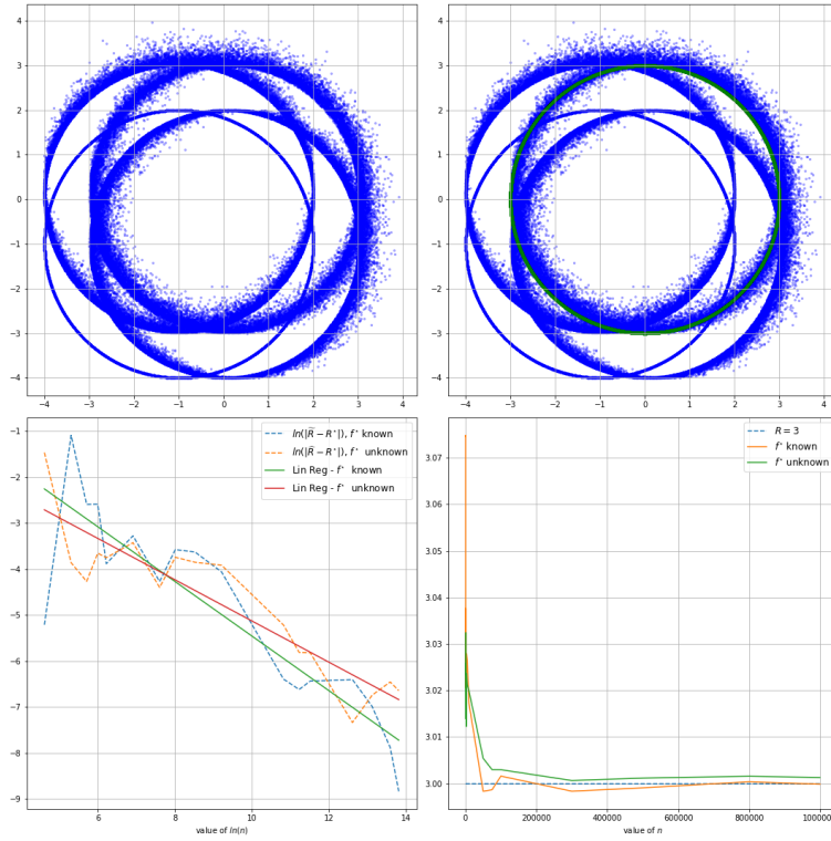
Figure 2: U \sim \text{Unif}(0,1) , for i \in \{1,2\} \varepsilon^{(i)} \sim \frac{1}{2}\delta_{(-1)} + \frac{1}{2}\mathcal{E}\text{xp}\left\{\frac{1}{0.12}\right\} and W = \{300, 400, 500, 1000, 2000, 3000, 5000, 10000, 50000, 75000, 100000, 300000, 500000, 800000, 1000000\}
