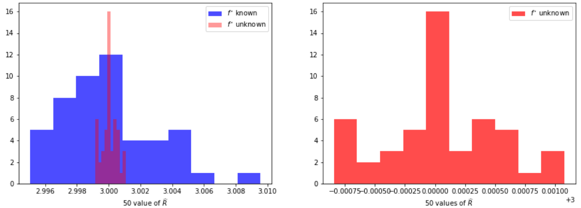
Figure 5: U \sim \text{Unif}(0, 1) and \varepsilon \sim \mathcal{N}(0, (0.12)^2 I)
