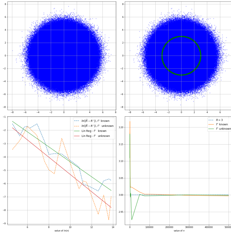
Figure 3: U \sim \text{Unif}(0,1) , \varepsilon \sim \mathcal{N}(0,1) and W = \{300, 400, 500, 1000, 2000, 3000, 5000, 10000, 50000, 75000, 100000, 300000, 500000\}
