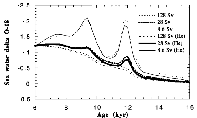
Fig. 5. Comparison of the seawater \delta^{18}\text{O} variations corresponding to the melting of an isotopically homogenous and an heterogeneous ice sheet for three different rates of ocean circulation (8.6 Sv, 28 Sv, and 128 Sv).
