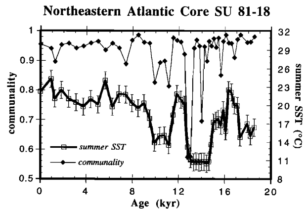
Fig. 1. Summer Sea Surface Temperature and faunal communality records from Northeastern Atlantic core SU 81-18.
