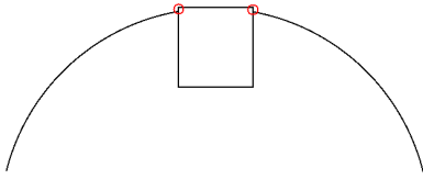
Fig. 22 Schematic of the integration problem
