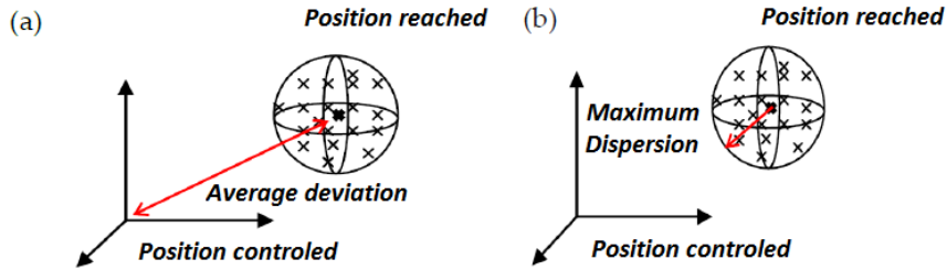
Figure 1: Accuracy (a) and repeatability (b) according to ISO 9283:1998
