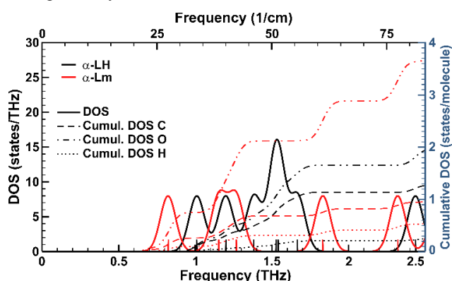
Figure 6. The \Gamma -point vibrational DOS of the hygroscopic \alpha -Lactose molecular crystal (black) and gas-phase \alpha -Lactose molecule (red), as obtained from the periodic calculations. The exact positions of the vibrational modes are indicated with the vertical black and red lines. A Gaussian smearing of 0.05THz was employed to generate the DOS. The cumulative atom-projected DOS for the different atomic species is indicated by the black (crystal) / red (gas-molecule) dashed (C), dash-dotted (O), and dotted (H) curves, respectively.
