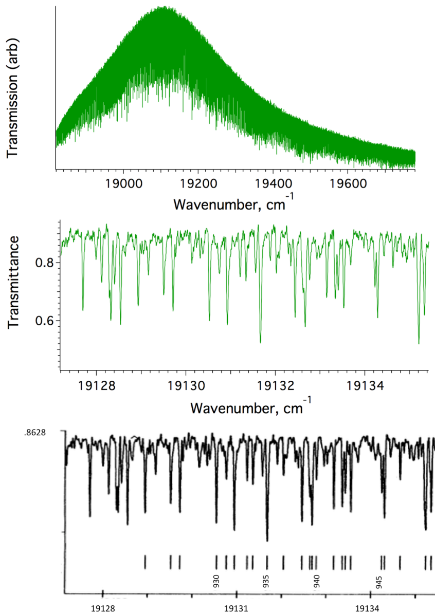
Figure 1. Illustration of the portion of the Tellurium absorption spectrum recorded through a combination of a blue-green filter (Corning glass 5-61) and a narrow-pass filter centred at 506 nm. The upper trace shows the raw absorption spectrum. The middle trace shows an 8 \text{ cm}^{-1} window in the corresponding transmittance spectrum. The lower trace displays a scan of the same region from the paper atlas of ref. 1 for comparison, reproduced with permission from Laboratoire Aimé Cotton.
