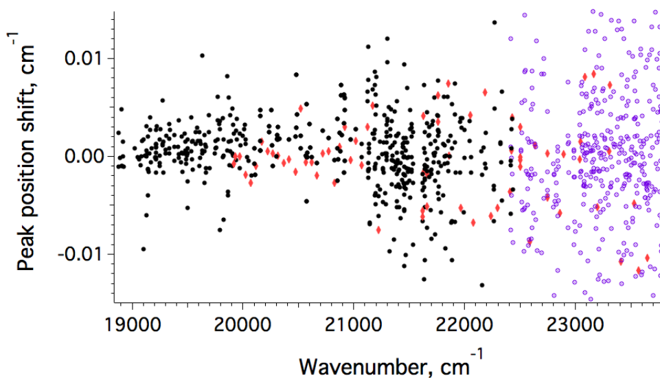
Figure 2. Scatter plot showing differences in \text{cm}^{-1} between peak positions determined as zero derivatives in our spectrum minus reference peak positions. Circles refer to the Doppler limited atlas 1 , diamonds (red) are shifts from the sub-Doppler values 6-8 . Open (violet) circles are from the lower-resolution spectra recorded with the UV beamsplitter.
