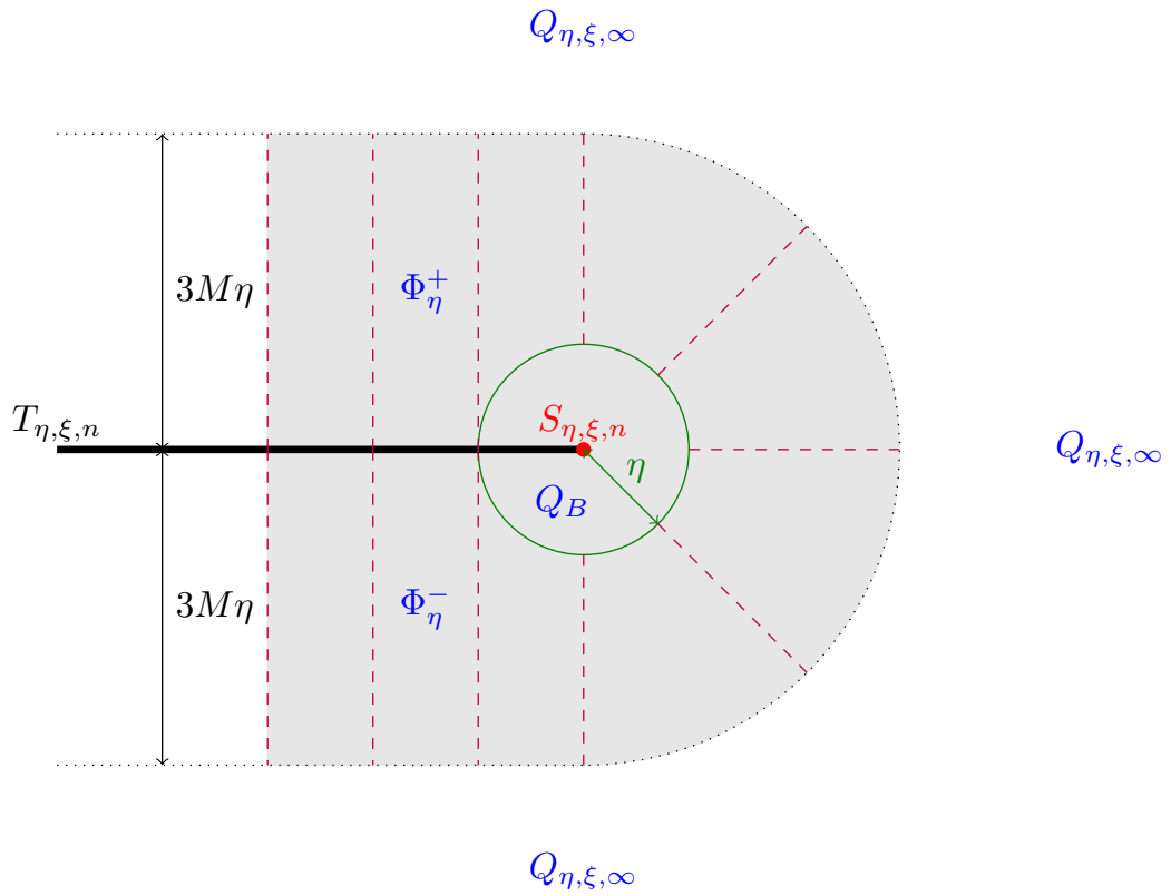
Figure 7: Sketch of the construction for Q_{\eta, \xi, n} in Step 4 in the region S_{3M\eta} defined in (86) (grey shaded area). Dashed lines indicate the direction of the projection \Pi .
