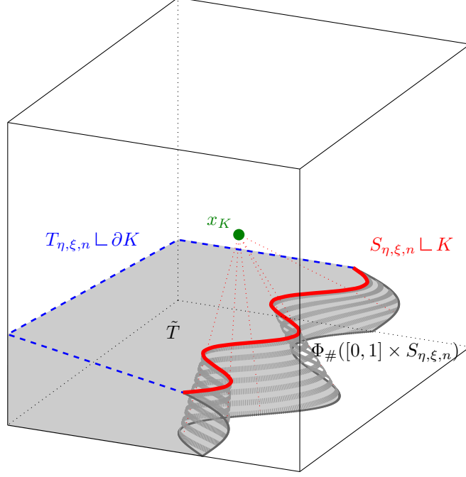
Figure 4: Construction near the boundary inside a cube: The newly created area (grey) is controlled by the surface of the cube and the length of the line singularity (red).
