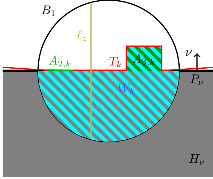
Figure 5: Schematic illustration of the quantities involved in Step 2 of the blow up procedure for T .
