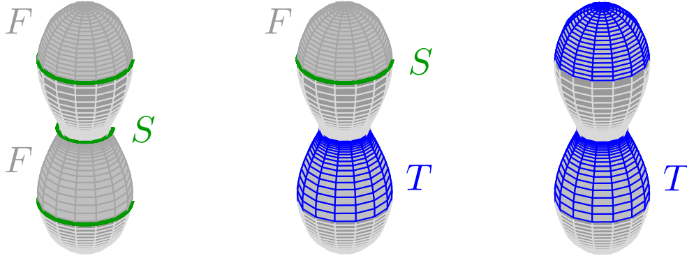
Figure 3: Expected minimizers of \mathcal{E}_0 for \beta \ll 1 (left), \beta \gg 1 (right) and intermediate \beta (center). For small \beta the line S has the tendency to stick to \mathcal{M} and optimize F , thus no T appears. Here, S = \Gamma and F consists of two connected components bounded by the three components of S . This configuration corresponds to three Saturn rings around the particle. For intermediate \beta one may find a configuration as depicted in the middle, i.e. the energy is decreased by joining two parts of S by a surface T glued to \mathcal{M} . This leads to the disappearance of the two rings that have been connected by T , and F contains only the part of \mathcal{M} above S . Finally, for large \beta , the last ring disappears and we obtain a dipole configuration in which S = \emptyset , F = \emptyset and T has two components, see Remark 3.4. This last configuration has been observed experimentally, see [73, Fig. 2(a)-(c)].
