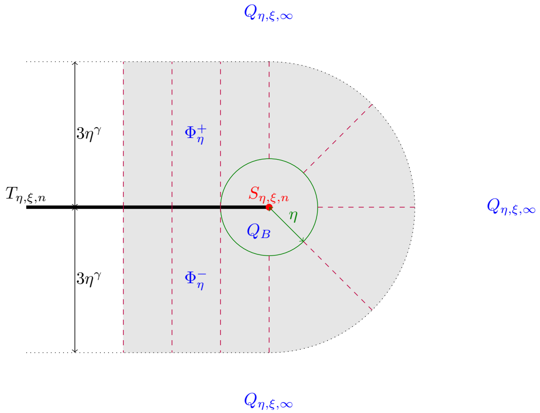
Figure 5: Sketch of the construction for Q_{\eta, \xi, n} in Step 5 in the region S_{3\eta^\gamma} defined in (63) (grey shaded area). Dashed lines indicate the direction of the projection \Pi .
