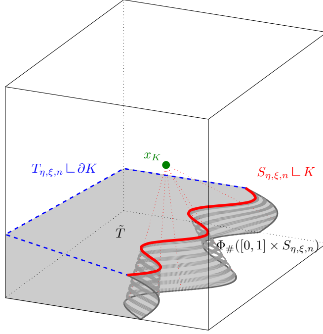
Figure 4: Construction near the boundary inside a cube: The newly created area (grey) is controlled by the surface of the cube and the length of the line singularity (red).
