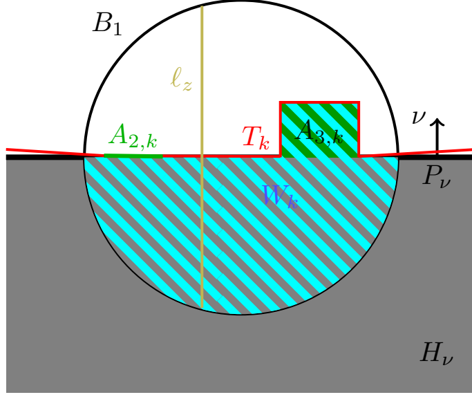
Figure 5: Schematic illustration of the quantities involved in Step 2 of the blow up procedure for T .
