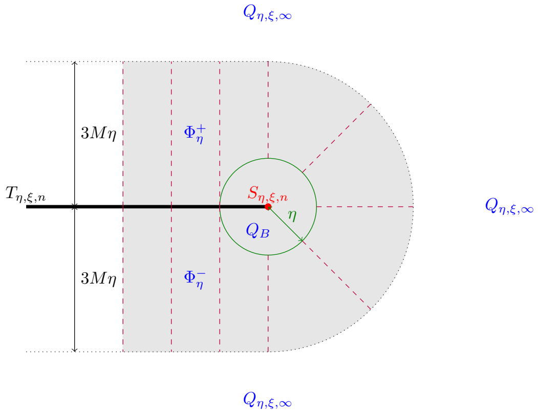
Figure 7: Sketch of the construction for Q_{\eta, \xi, n} in Step 4 in the region S_{3M\eta} defined in (87) (grey shaded area). Dashed lines indicate the direction of the projection \Pi .
