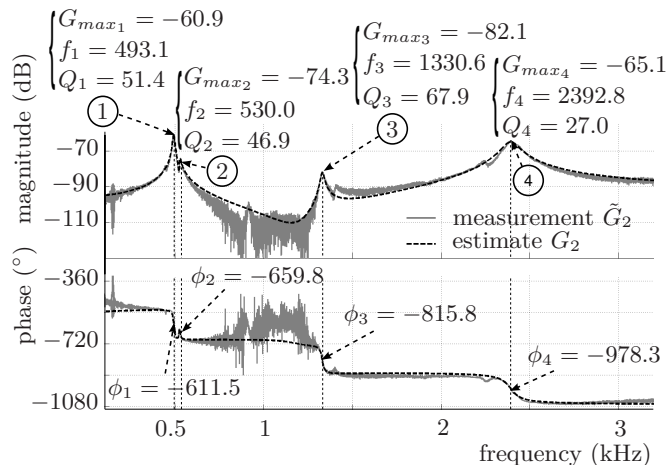
Figure 3: Measurement \tilde{G}_2 and estimate G_2 of the frequency response of the system {xylophone bar + transducers}.
