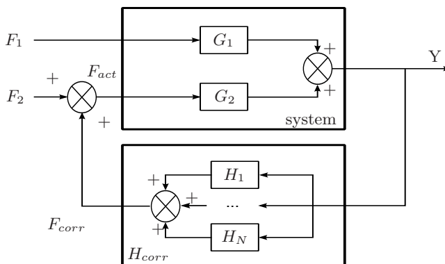
Figure 1: Diagram of the closed-loop system, described by the frequency responses G_1 and G_2 and by the controller response H_{corr} .
