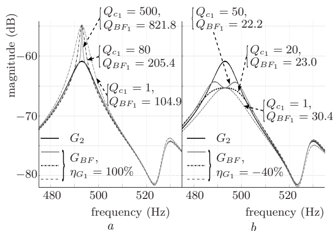
Figure 6: The controllers are intended to modify the bandwidth of peak 1, namely \Delta_{\omega_1} , and to increase its amplitude by +100\% first (a), and to reduce it by 40\% (b) then. Its frequency is unchanged. The quality factor Q_{BF_1} is estimated by the \omega_1/\Delta_{\omega_1} ratio.
