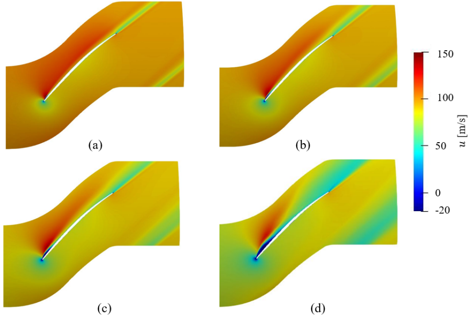
Figure 6: Contours of averaged streamwise velocity u around rotor blade, for various mass flow rates, (a) \dot{m} = 22 kg/s, (b) \dot{m} = 21 kg/s, (c) \dot{m} = 20 kg/s and (d) \dot{m} = 19 kg/s.
