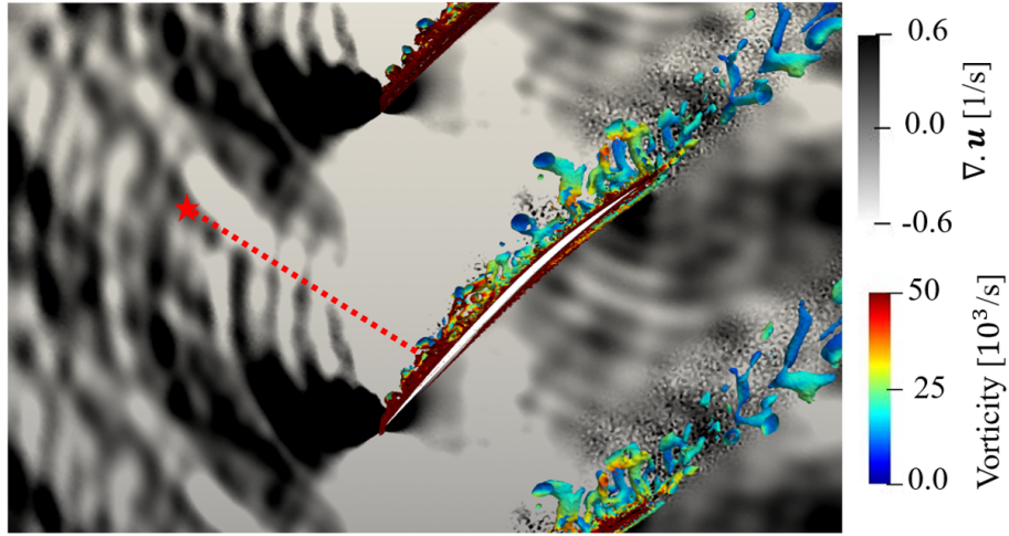
Figure 13: Instantaneous contours of dilatation rate and iso-surfaces of Q-criterion ( Qc^2/U_0^2 = 100 ) colored by the vorticity magnitude at \dot{m} = 20 kg/s. The star symbol indicates the location of the monitor point where unsteady pressure samples were collected for the PSD computation. The dashed-line shows the location of the monitor points used for the calculation of the coherence.
