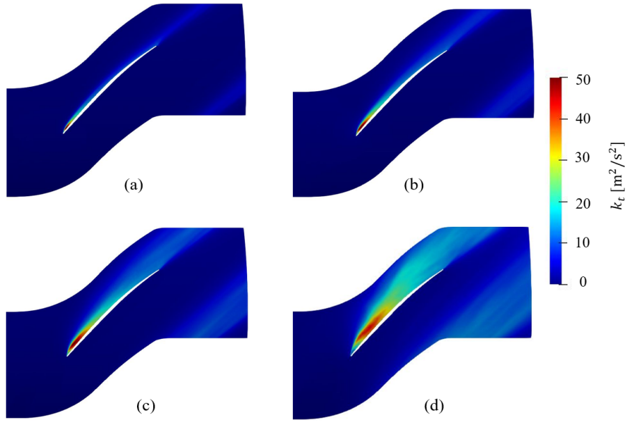
Figure 7: Contours of turbulent kinetic energy k_t around the rotor blade, for various mass flow rates, (a) \dot{m} = 22 \text{ kg/s} , (b) \dot{m} = 21 \text{ kg/s} , (c) \dot{m} = 20 \text{ kg/s} and (d) \dot{m} = 19 \text{ kg/s} .
