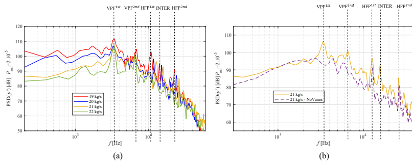
Figure 14: PSD of the pressure fluctuations from a monitor point normal to the rotor surface at one chord length from the rotor LE. (a) Rotor-stator simulations at various mass flow rates. (b) comparison with a rotor-only simulation at \dot{m} = 21 kg/s.
