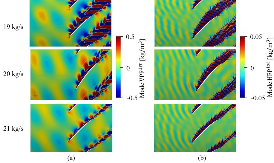
Figure 15: Spatial distribution of the density modes using the DMT technique. (a) \text{VPF}^{1st} . (b) \text{HFP}^{1st} .
