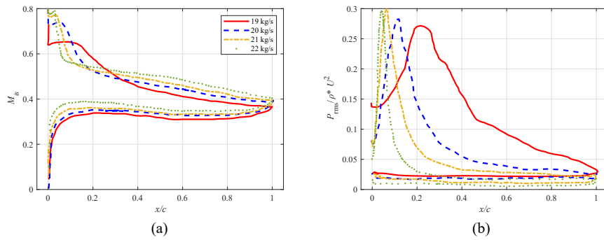
Figure 8: Average isentropic Mach number M_{i,s} (a) and RMS pressure fluctuations P_{rms} (b) along the rotor blade for various mass flow rates.
