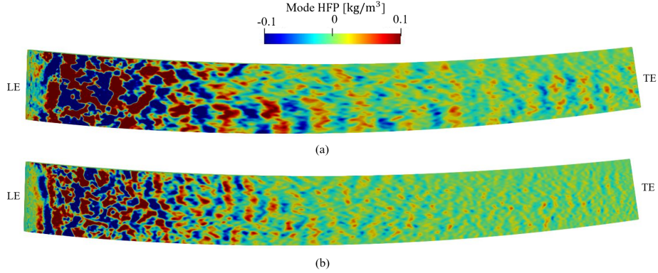
Figure 17: Spatial distribution of the density modes using the DMT technique on the suction side of the rotor blade at \dot{m} = 19 kg/s. (a) HFP 1st . (b) HFP 2nd .
