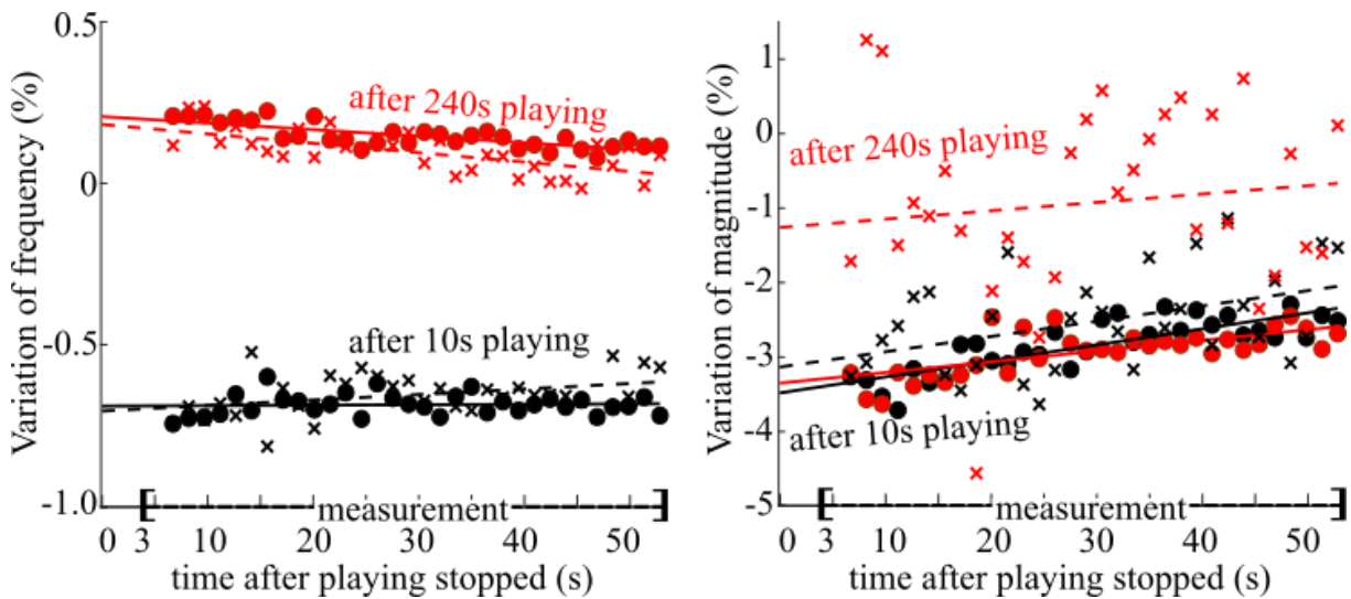
FIG. 2. Examples of the extrapolation procedure used to estimate the percentage changes in the frequencies f_{\text{max}} and f_{\text{min}} , and the magnitudes Z_{\text{max}} and Z_{\text{min}} of the extrema in Z_{\text{bore}} at the moment playing ceased ( t = 0 ). The percentage variations in frequency (left) and magnitude (right) of the impedance maxima and minima over the measurement period are relative to the values measured before playing started. Circles indicate the average values of peaks 3 to 7 (169 Hz to 405 Hz) for each cycle and the crosses indicate the average values of minima 3 to 7 (195
