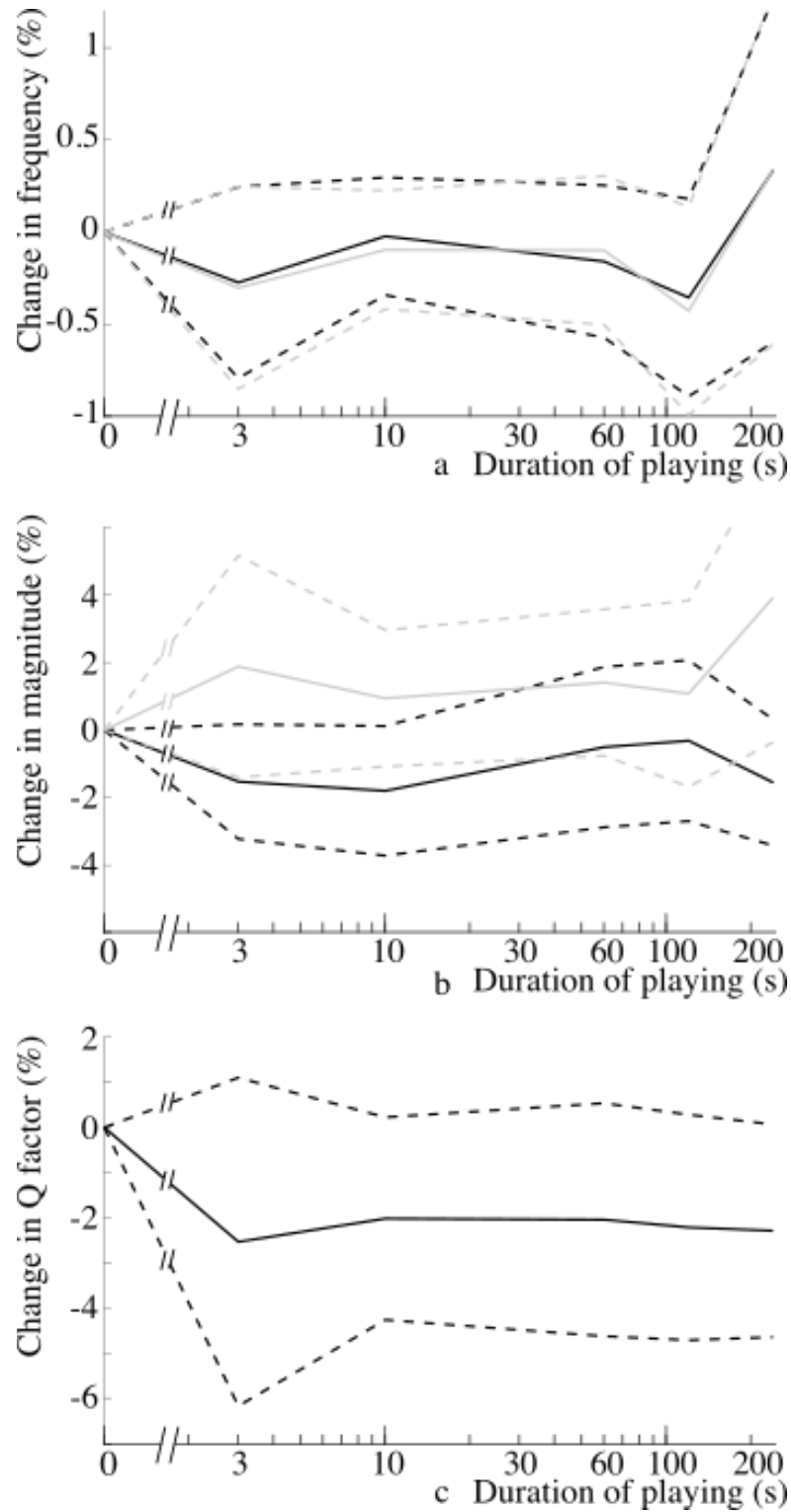
FIG. 6. The mean percentage changes in the frequencies (a), magnitudes (b) of the extrema in Z_{\text{bore}} and Q factors (c) of impedance peaks 3 to 7 versus duration of playing (on a log scale), in a lab at 39°C and 45% relative humidity. The black and gray lines (top and middle) show the variations of the corresponding impedance maxima and minima respectively. The dashed lines
