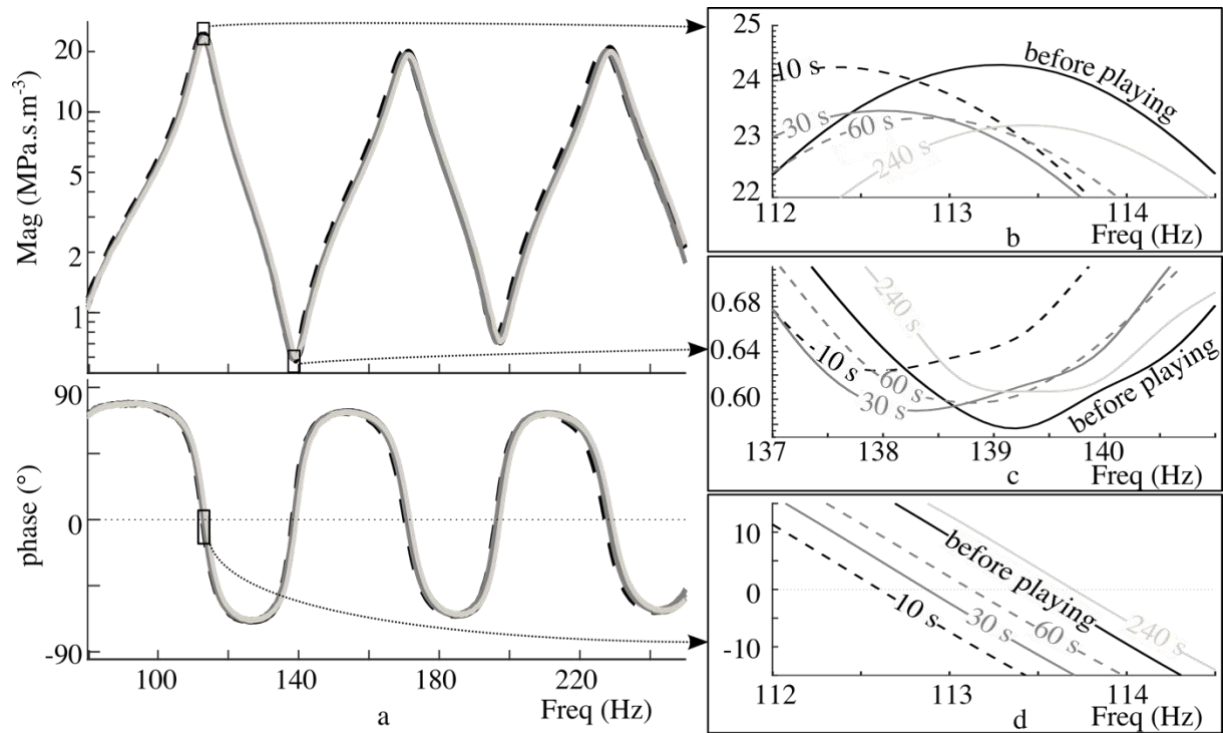
FIG. 3. A section of Z_{\text{bore}}(f) measured 3 s after different durations of playing by the same player (a). The insets zoom in on the impedance magnitude maxima (b) and minima (c) and on the phase zero-crossing (d) of the first resonance shown (the second impedance peak for the instrument).
