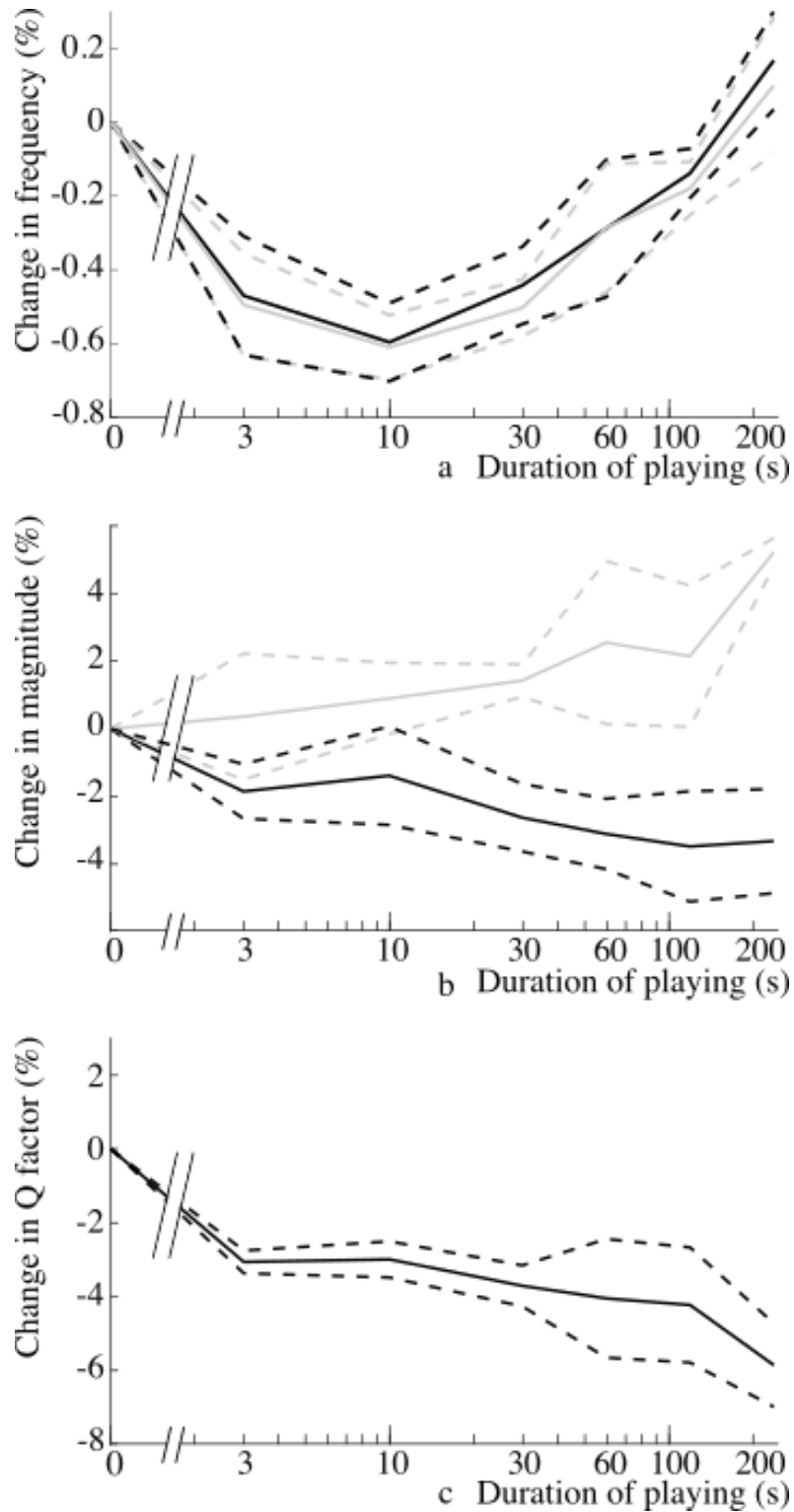
FIG. 4. The mean percentage changes in the frequencies (a), magnitudes (b) of the extrema in Z_{\text{bore}} and Q factors (c) of impedance peaks 3 to 7 versus duration of playing (on a log scale), in a lab at ambient temperature and 55% relative humidity. The black and gray lines (top and middle) show the variations of, respectively, the corresponding impedance maxima and
