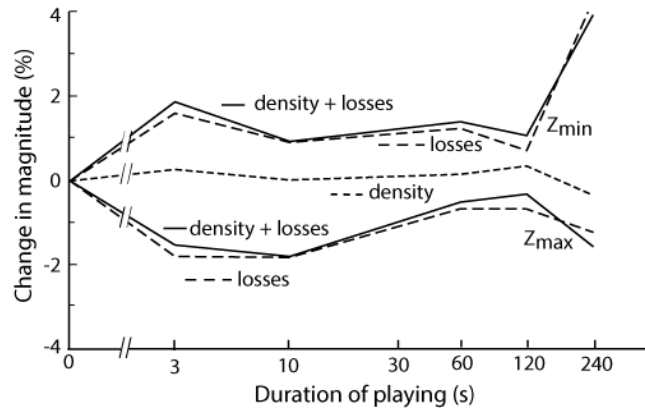
FIG. 7. Separation of the percentage changes in the mean values of Z_{\max} and Z_{\min} into those caused by density changes and those caused by changes in the losses, at 39 °C.
