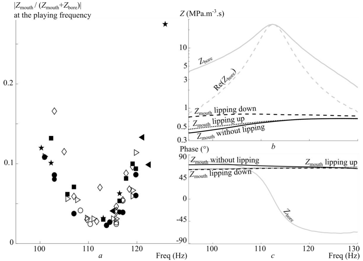
FIG. 2. a : (left) Impedance ratios |(Z_{\text{mouth}}/(Z_{\text{mouth}} + Z_{\text{bore}}))| at the playing frequencies near B \flat 2 (nominally 116.5 Hz) for the seven players. Each symbol shows one measurement. The open symbols correspond to beginners. (right) – Measured bore impedance (magnitude and real part (b), and phase (c) (gray curves) and mouth impedances (black curves) averaged for all players while playing at normal pitch (solid), while lipping down (dashed) and while lipping up (dotted).
