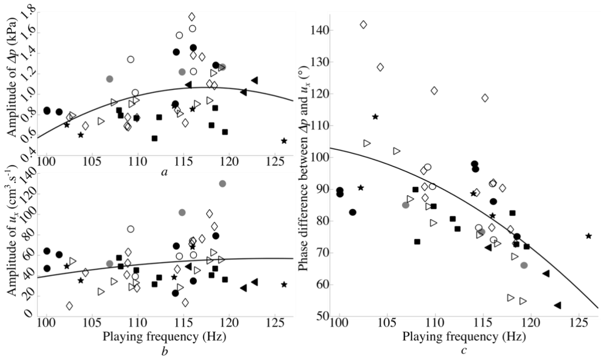
FIG. 7. Amplitude of the acoustic pressure difference \Delta p across the lips (a), of the acoustic component of the longitudinal sweeping flow u_x (b) and phase difference between \Delta p and u_x (c), versus playing frequency for advanced players (closed symbols) and beginners (open symbols). The solid black lines show quadratic regressions. The grey symbols are for the examples in Figs 3 and 4.
