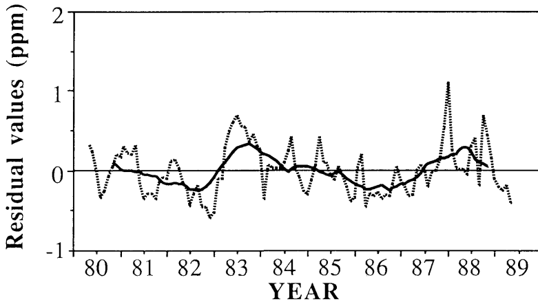
Fig. 2. Difference r(t) between the observed monthly mean concentrations ( y(t) ) and the 4th degree polynomial P_4(t) (dotted curve), and the corresponding smoothed spline (solid curve ( L(t) )) calculated by means of a 12-month running mean of r(t) .
