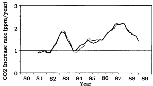
Fig. 7. Increase rate of the atmospheric CO 2 concentrations. The solid curve is obtained with all 222 Rn data. The dotted curve is obtained with data when 222 Rn < 1 pCi m -3 .
