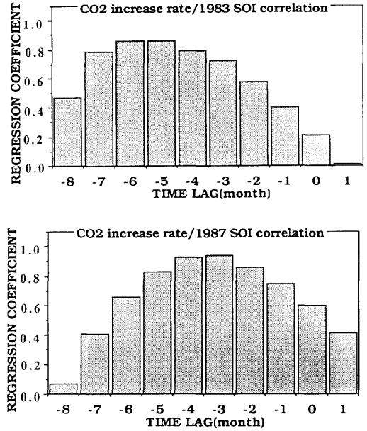
Fig. 4. Lag correlations between the CO 2 increase rate and SOI in 1983 (top) and 1987 (bottom).
