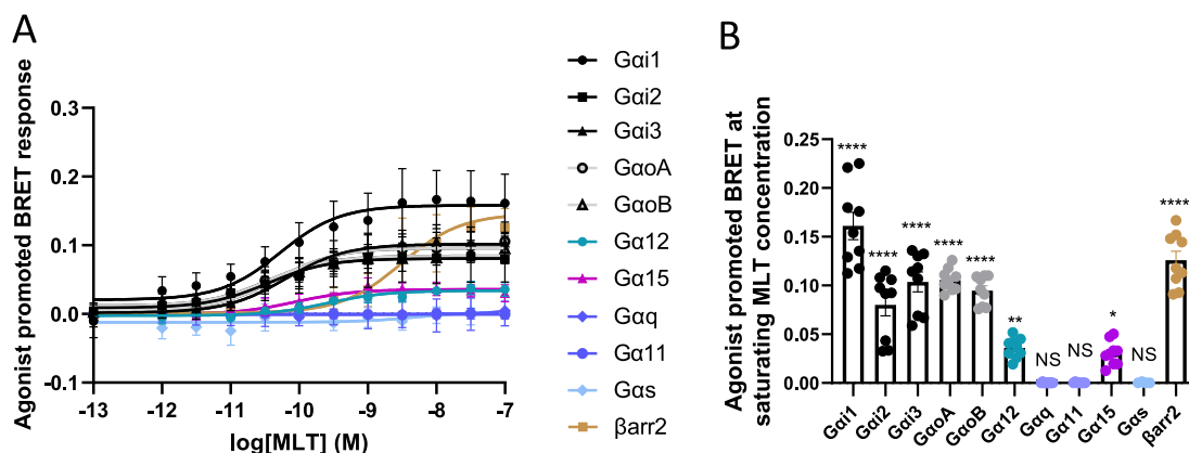
Figure 1. MT 1 -WT activates Gai/o , Gα12 , Gα15 , and recruits βarrestin-2 . (A) MLT concentration curves for MT 1 -WT. Data were plotted using nonlinear regression curves with a fixed Hill slope equal to 1. (B) MT 1 response for Gai1 , Gai2 , Gai3 , GaoA , GaoB , Gα12 , Gαq , Gα11 , Gα15 , and Gαs activation and βarrestin-2 recruitment at saturated MLT concentration (100 nM) of the corresponding curves in A. Statistical analysis was performed using one-way ANOVA followed by a Dunnett's posthoc test. Data represents the mean ± SEM of 5 to 9 experiments. Data were fitted in GraphPad Prism 9. * p \leq 0.05 , ** p \leq 0.01 , **** p \leq 0.0001 . βarr2 : βarrestin-2 .
