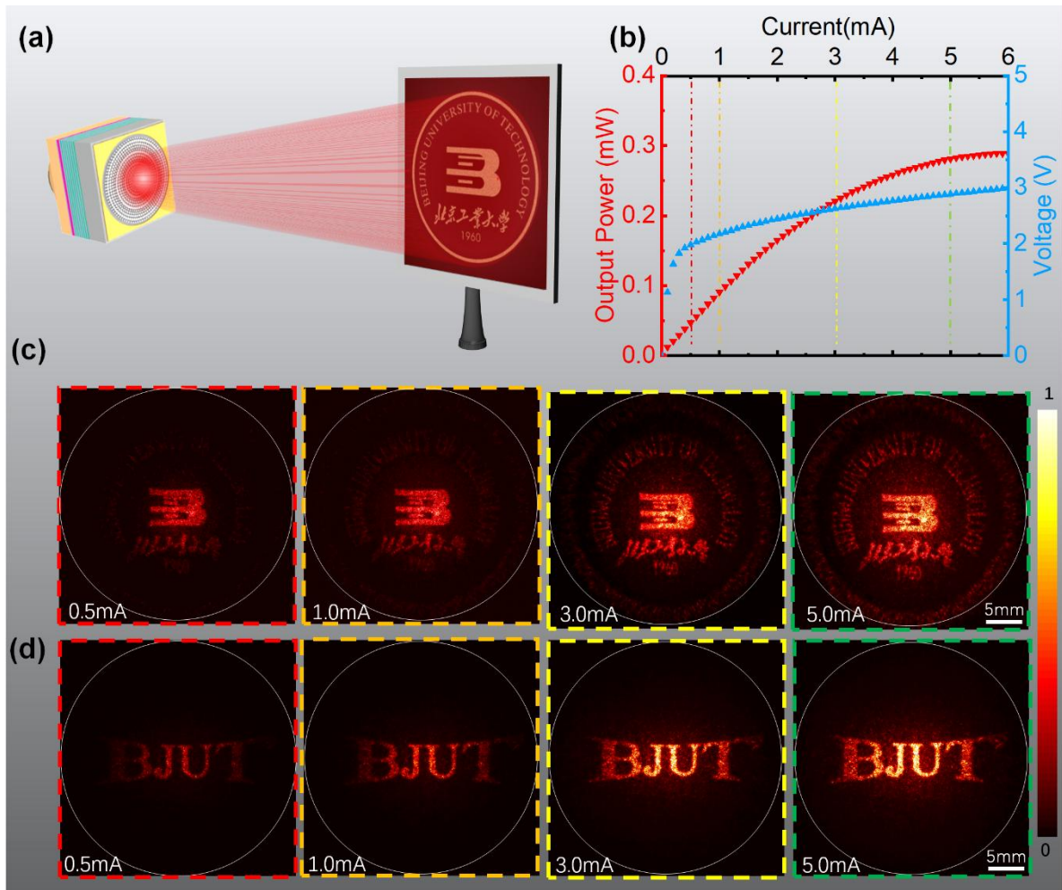
Figure 4. Wafer-level holographic beam structuring with large field of view. a) Schematic illustration of a holographic MS-VCSEL for the construction of complex beam patterns, in this example, an infrared image of university logo is constructed and directly projected onto a screen for observation. b) The P - I - V characteristics confirm that the holographic MS-VCSEL has comparable performance as the bare laser prior to the integration of holographic metasurface. c) and d) Experimentally reconstructed images directly from two different holographic MS-VCSELs under 0.5, 1, 3, and 5 mA, respectively, showing that the intensity of the image increases as the injection current increases and more features can be resolved at higher current. The scale bar is 5 mm.
