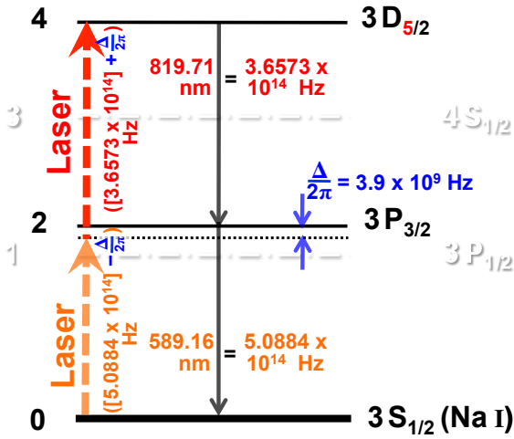
Figure 1. Atomic level diagram (not to scale) for neutral sodium atoms in the two-laser LPRS technique described in this paper. The allowed transitions and levels (i.e., levels 0, 2, and 4 in the diagram) are in solid black, whereas a dotted black line represents the off-resonant energy corresponding to the frequency of the first laser. The 5 in the allowed 3D_{5/2} level is red to distinguish this atomic state from the 3D_{3/2} Na I state that is excited by the 343 nm laser in the technique described in Paper I. The two “ghost” levels (1 and 3) below the 3D_{5/2} excited state, that are both inaccessible from states in the diagrams that are excited by the lasers, are shown in shadowed gray text and dash-dotted lines. As is shown, this LPRS technique results in a “fully-mandated cascade” from the 819.71 nm de-excitation to the 589.16 nm de-excitation, resulting in a mandated 1:1 ratio between those produced photons.
