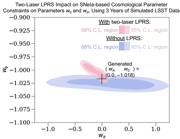
Figure 3. Constraints on the dark energy equation of state parameters w_0 and w_a , obtained using simulated catalogues of type Ia supernovae. Each one of the two SNeIa catalogues that are fitted to obtain these constraints contains 120000 simulated SNeIa (corresponding to approximately 3 years of observation at the Rubin Observatory). The generation of the two simulated SNeIa catalogs, as well as the fits that are performed to each catalog, are implemented using the CosmoSIS cosmological parameter estimation code (Zuntz et al. 2015), and are explained in the text here, as well as in Section 9 of Paper I. The resulting values of the figure of merit parameter \mathcal{F}_{\text{DE}} for the fits are 313 for the fit to the SNeIa catalog representing expected LSST observations without LPRS-based photometric calibration, and 1646 for the fit to the SNeIa catalog representing expected LSST observations with photometric calibration from the two-laser LPRS described in this paper. (Also, as would be expected on average, the central values of each fit are approximately one standard deviation away from the generated values of w_0 and w_a .) The fits represent a \frac{1646}{313} = 5.26 -fold expected improvement in the dark energy figure of merit parameter \mathcal{F}_{\text{DE}} from LPRS-based photometric calibration (with even greater expected resulting \mathcal{F}_{\text{DE}} increases for SNeIa datasets that correspond to greater than 3 years of Rubin Observatory observation).
