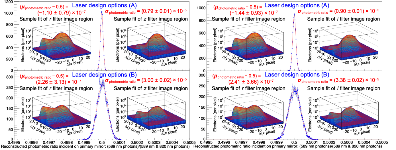
Figure 2. Within each of the four sets of plots above, the main plot (i.e., the 1-dimensional fitted Gaussian curve in the centre of each set of plots) shows the distribution of 10000 fitted photometric ratios, with each ratio reconstructed from pairs of simulated r and z filter image regions (within the two sets of plots on the left-hand side above), and pairs of simulated r and i filter image regions (within the two sets of plots on the right-hand side above). Within both the left-hand and right-hand sets of plots, the upper set of plots shows the results of fits with image regions simulated when assuming that the LPRS is generated with laser design options (A), with specifications detailed in Section 4; and the lower set of plots shows the results when assuming that the LPRS is instead generated with laser design options (B). Within each of the four sets of plots, each one of the respective 2 \times 10000 simulated image regions consists of a 50 \text{ pixel} \times 50 \text{ pixel} square centered around the observed LPRS centroid. The inset plots show single examples of simulated r and z image regions (within the two sets of plots on the left), and simulated r and i image regions (within the two sets of plots on the right), with their respective fits to 2-dimensional Gaussian LPRS signal ellipses, plus the product of a falling exponential along the x -axis and a Gaussian distribution along the y -axis to parametrize the tail of the trail of Rayleigh-scattered background laser light that “leads up” to the LPRS spot (which is perhaps reminiscent of an “entrance to an igloo” in all of the inset plots), plus flat background distributions. These inset plots all have a logarithmic z -axis, and linear x - and y -axes. The simulated signal photoelectrons, Rayleigh background photoelectrons, and sky + noise background photoelectrons, in each simulated pixel within each region, are generated according to the statistical distributions expected from a single 30 s LSST visit consisting of a pair of 15 s exposures. The fitted number of signal photoelectrons is extracted from each image region fit, and divided by the (photoelectron)/(incident photon) efficiency (consisting of the expected LSST detector quantum efficiency, multiplied by the expected throughput fraction of telescope, camera, and filter optics, at 589 nm and at 820 nm for the simulated r , z , and i filter image regions respectively), to determine the reconstructed numbers of 589 nm and 820 nm photons incident on the Rubin Observatory primary mirror during the 30 s visit. For each simulated image region pair, the resulting ratio of reconstructed (589 nm photons)/(589 nm photons + 820 nm photons) is plotted, and the resulting distribution is fitted to a single Gaussian. The standard deviations of the fits shown in the main plots within the two left sets of plots above, which correspond to the expected LPRS photometric ratio statistical uncertainties from a single pair of visits with the r and z filter, are equal to (0.79 \pm 0.01) \times 10^{-5} in the case of an LPRS that is generated according to laser design options (A), and to (3.00 \pm 0.02) \times 10^{-5} in the case of an LPRS that is generated according to laser design options (B). The standard deviations of the fits shown in the main plots within the two right sets of plots above, which correspond to the expected LPRS photometric ratio statistical uncertainties from a single pair of visits with the r and i filter, are equal to (0.90 \pm 0.01) \times 10^{-5} in the case of an LPRS that is generated according to laser design options (A), and to (3.38 \pm 0.02) \times 10^{-5} in the case of an LPRS that is generated according to laser design options (B). The means of the fits that are shown in the main plots within all four of these sets of plots are all consistent with 0.5.
