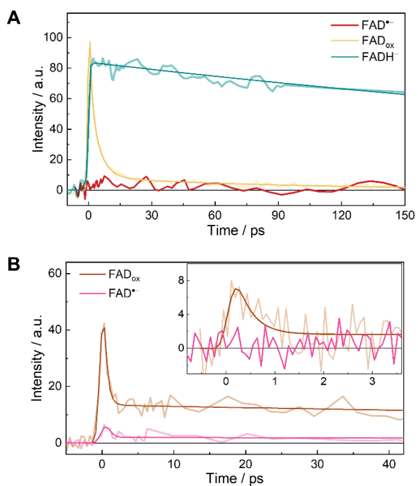
Figure 2. (A) Fluorescence decays of FAD •- , FAD ox , and FADH in GOX monitored at 537 nm under the same excitation conditions with CS 2 as the Kerr medium. Intensities were normalized based on the absorption of the samples at the excitation wavelength (390 nm). (B) Fluorescence decays of the as-prepared aerobic (FAD ox ) and reduced (FAD •- ) samples of COX monitored at 532 nm, with benzene or suprasil (inset) as Kerr medium. Measurements were conducted with the same sample before and after the chemical reduction (see text). Exponential fits are shown as smooth curves.
