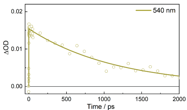
Fig. S11. Isotropic transient absorption kinetics of FADH - in GOX at 540 nm upon excitation at 390 nm.
