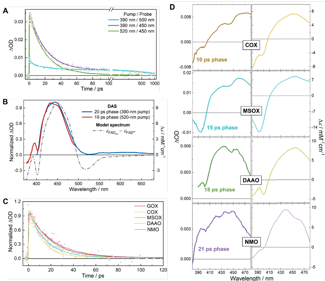
Figure 3. (A) Isotropic transient absorption kinetics of FAD^{\cdot-} in GOX at selected wavelengths upon excitation at 390 nm or 520 nm. (B) Spectral analysis of DAS of FAD^{\cdot-} in GOX under two excitation conditions. Model spectrum was constructed from steady-state spectra by assuming complete FAD^{\cdot-} to FAD_{ox} conversion. (C) Isotropic transient absorption kinetics in different flavoprotein oxidases after excitation at 520 nm and monitored at 455 nm. (D) DAS of anionic flavin radicals in COX, MSOX, DAAO and NMO under excitation at 520 nm, as well as the corresponding steady-state difference spectra.
