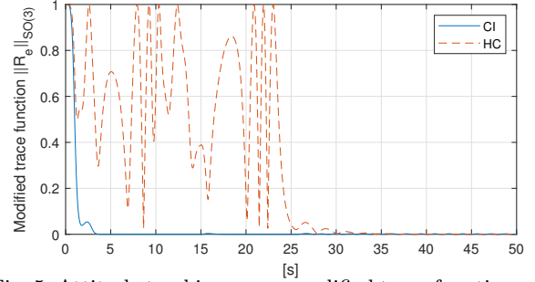
Fig. 5. Attitude tracking error: modified trace function when choosing K_R = 2I_3 ( \|R_e\|_{SO(3)} ).
