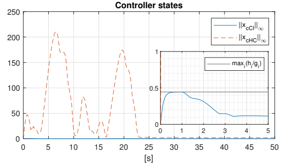
Fig. 6. Infinity norm of the controller states ( \|x_c\|_\infty = \max_i(|x_{c_i}(t)|) ).
