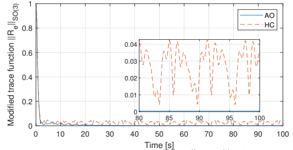
Fig. 7. Attitude tracking error ( \|R_e\|_{SO(3)} ). Adaptive Observer (AO) vs standard Harmonic Controller (HC).
