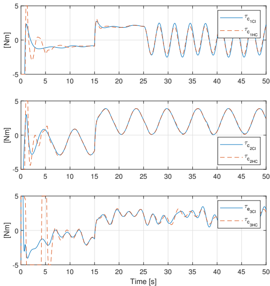
Fig. 4. Control torque: components of \tau_c .
