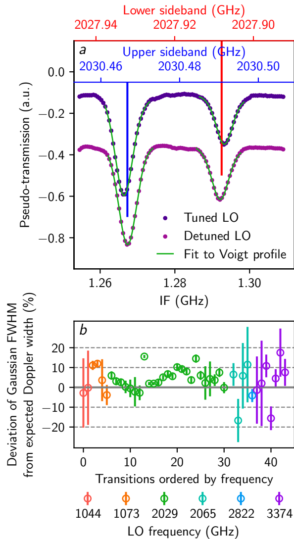
Fig. 3. a , the spectrum of methanol recorded by the heterodyne spectrometer with tuned QCL settings (purple, \nu_{\text{LO}} = 2029\text{GHz} ), and the same spectrum recorded after slightly detuning the QCL (magenta). Since the LO frequency is red-shifted after detuning, peaks in the IF that are also red-shifted must originate from the lower sideband. Alternatively, peaks in the IF that are blue-shifted must originate from the upper sideband. The methanol transitions from the JPL database (Ref. [29]) corresponding to the upper sideband (blue) and lower sideband (red) are indicated. Also included is a fit of a Voigt profile to the recorded peaks (green). The data has been smoothed and resampled by a factor of 1/7. b , The deviation in percent of the fit Gaussian FWHM value from the expected value (the calculated FWHM Doppler broadening with temperature = 292 K) for each fit methanol transition, coloured by the different LOs.
