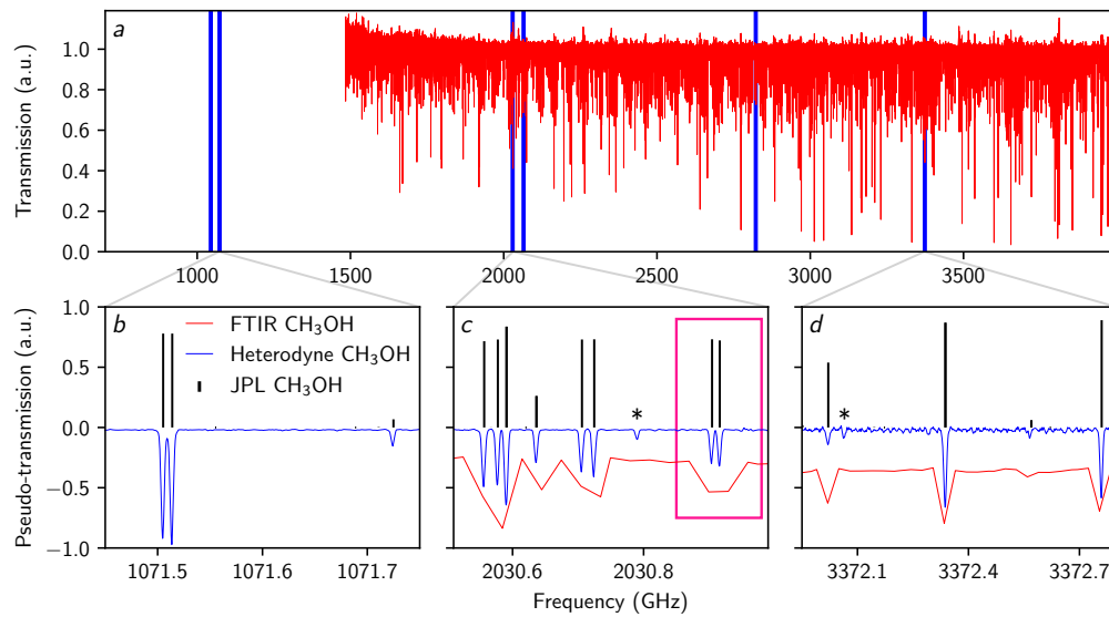
Fig. 2. Comparison of a methanol transmission spectrum recorded by the FTIR spectrometer with methanol pseudo-transmission spectra recorded by the THz heterodyne spectrometer. a. The FTIR spectrum below 4 THz (red) with the position of six LO frequencies used in the heterodyne THz spectrometer (blue lines). The broadband FTIR measurement is limited at the low-end to around 1500 GHz by reduced transmission of components in the instrument. b, c, d. Partial portions of spectra recorded by the THz heterodyne spectrometer (blue) at LO frequencies of 1073 GHz ( b ), 2029 GHz ( c ), and 3374 GHz ( d ) along with the FTIR spectrum (red). Peaks originating from the opposing sideband from the one displayed are marked with an asterisk. Transition frequencies of methanol taken from the JPL database are shown as black lines (Ref. [29]). Highlighted in pink in c is an example of a torsional fine splitting.
