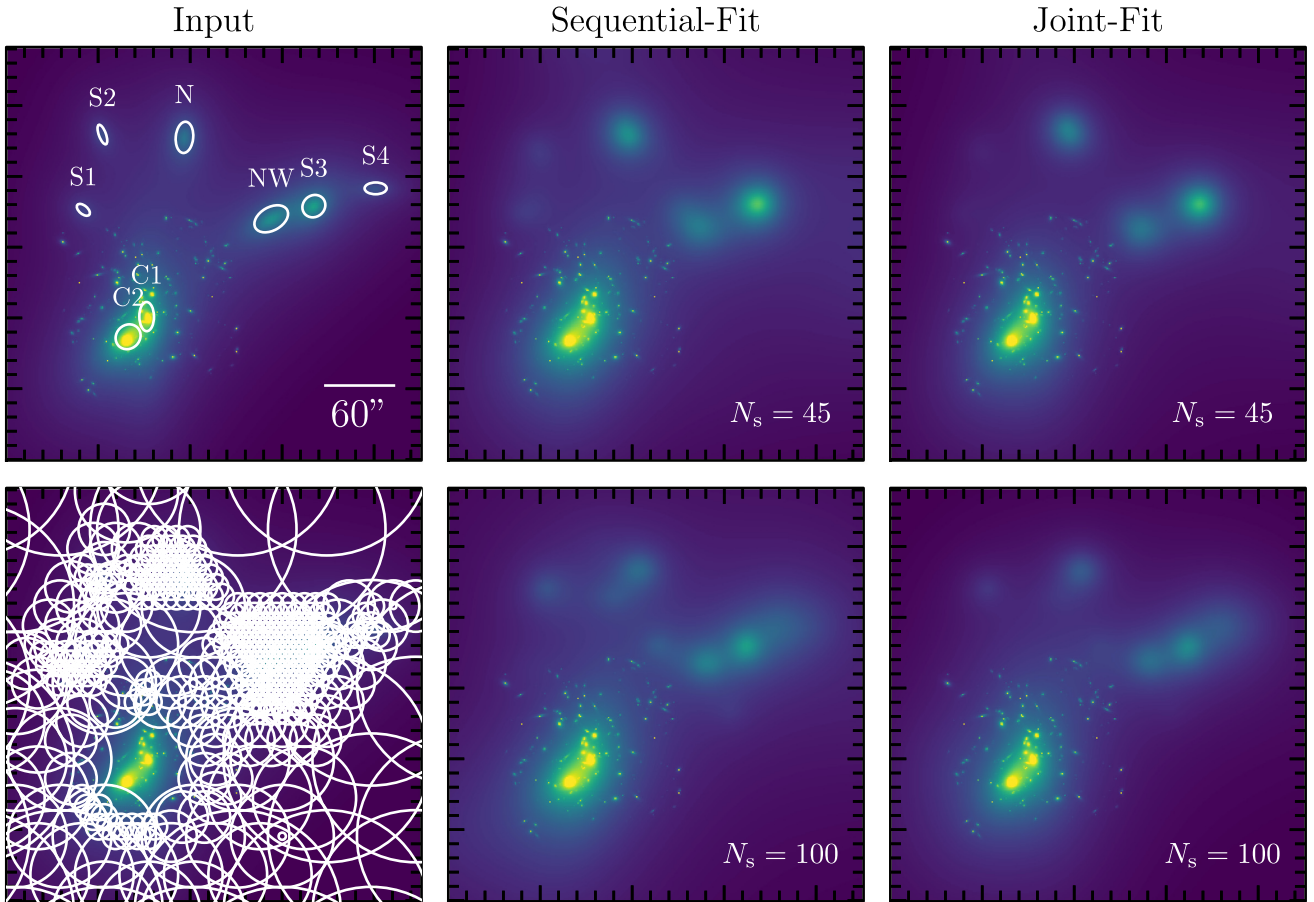
Figure 1. Projected mass maps. Left column: Input simulation, with the large-scale potentials shown as white ellipses (top panel), and the potentials of the multiscale grid shown as white circles, which sizes are set to the core radii, s , of the potential (bottom panel). Middle column: Sequential-Fit , with source density N_s = 45 sources arcmin ^{-2} (top) and N_s = 100 sources arcmin ^{-2} (bottom). Right column: Joint-Fit , with source density N_s = 45 sources arcmin ^{-2} (top) and N_s = 100 sources arcmin ^{-2} (bottom). The Sequential- and Joint-Fit mass maps are means over a 1000 MCMC samples.
