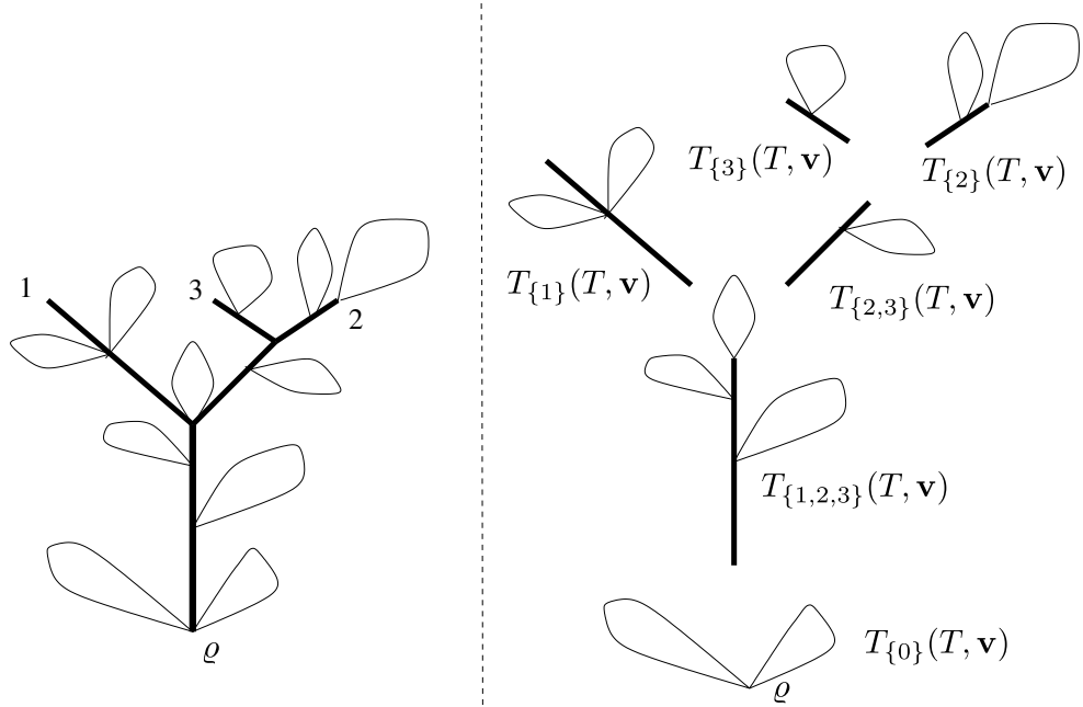
FIGURE 5. The splitting of the left hand tree with respect to \mathbf{v} = \{0, 1, 2, 3\} . In this instance, T_{\{1,2\}} and T_{\{1,3\}} are reduced to their own root.
