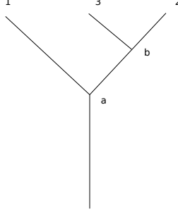
FIGURE 4. A discrete trees spanned by the leaves \{1, 2, 3\} .
