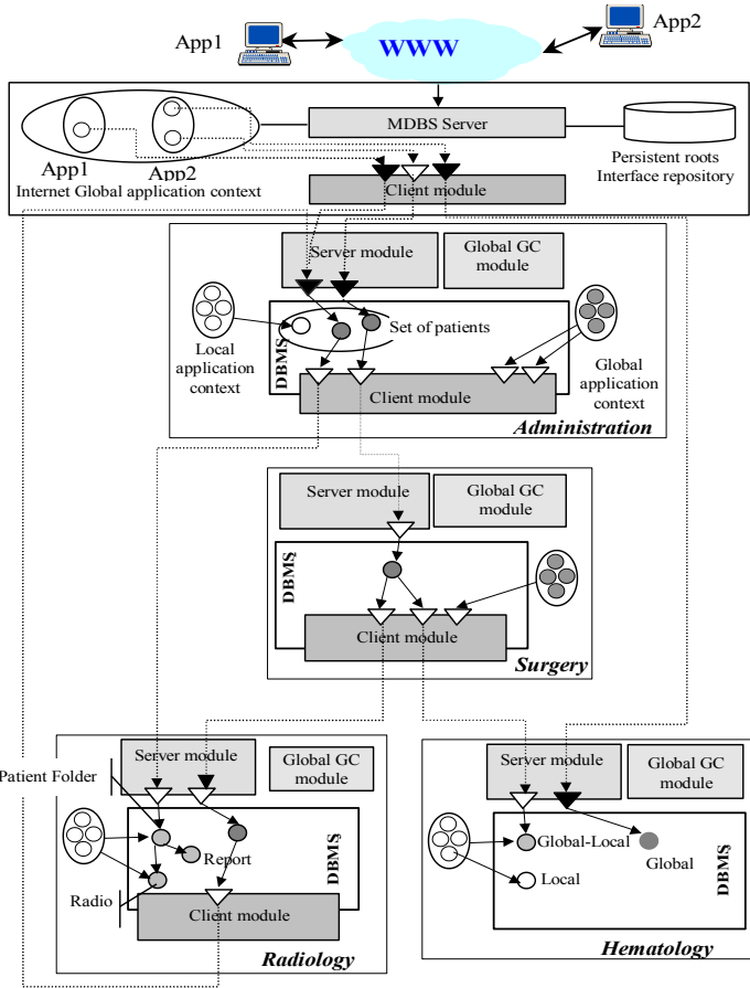
Figure 2: General Architecture
