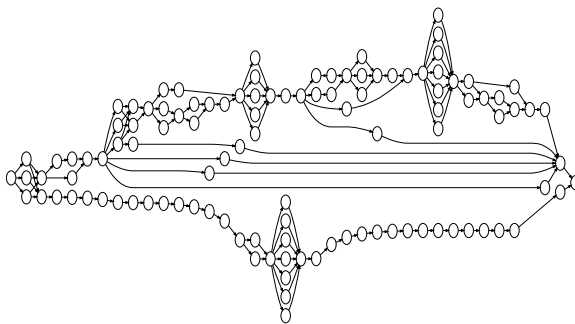
Figure 1: A DAG representing game engine tasks (vertices) and their precedence constraints (edges, from left to right).
