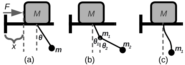
Fig. 1. (a) single-pendulum, (b) double-pendulum, (c) flexible-cable
