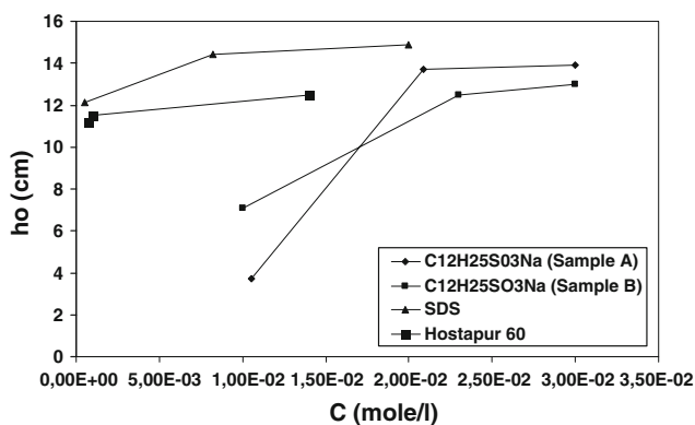
Fig. 1 Height of the foam versus the concentration of sodium dodecanesulfonates (samples A and B), Hostapur 60 and sodium dodecylsulfate at 25 °C
