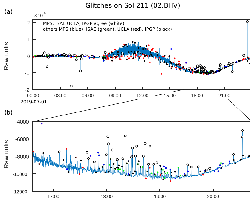
Figure 2. (a) Comparison between glitches detected on 02.BHV (VBB) on 1 July 2019 (Sol 211) by our four groups: MPS, ISAE, IPGP, and UCLA. White circles are commonly detected glitches for all groups. Color-coded symbols correspond to glitches for the different groups that are not common to all. Those common to subgroups are plotted on top of each other and so the last plotted is shown. (b) Expanded section showing that as the threshold for declaring a glitch is lowered, either in terms of signal-to-noise or correlation with the template, the results differ and a few, small candidate glitches have been missed.
