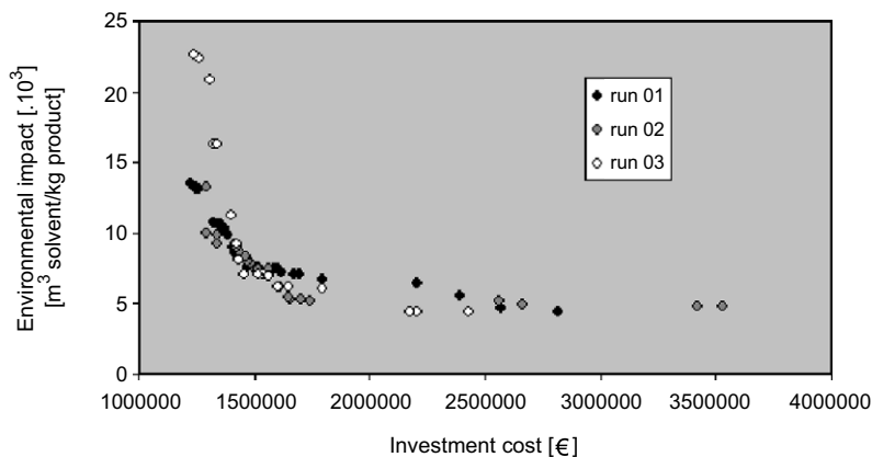
Fig. 11. Pareto's optimal solutions for solvent used – investment cost, Policy A (monoproduct).
