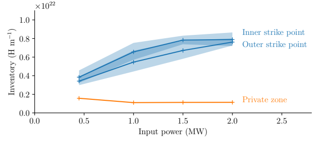
(a) Inventory per unit thickness after 10^7 \text{ s} of exposure. The area corresponds to the 95% confidence interval.
