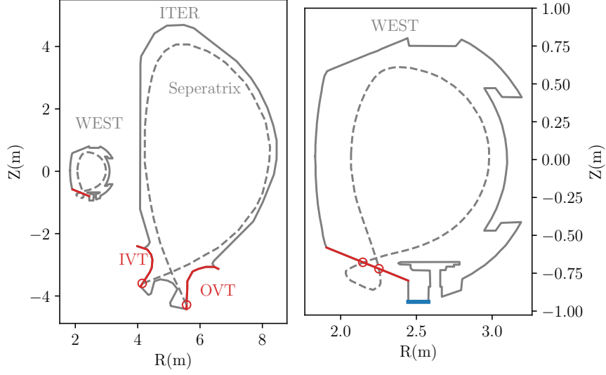
Figure 1: Geometry of WEST and ITER divertors showing the divertors in red, the plasma separatrix and the location of the strike points. IVT and OVT stand for Inner and Outer Vertical Target, respectively. For WEST, the pump position (in blue) is under the baffle.
