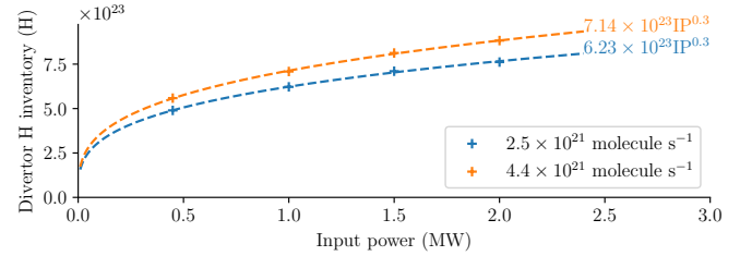
Figure 7: Evolution of the WEST divertor inventory as a function of SOL input power (IP) for several puffing rates.
