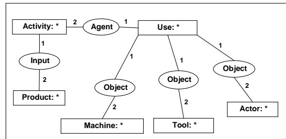
Figure 8. Example of generic CG for the context's description
