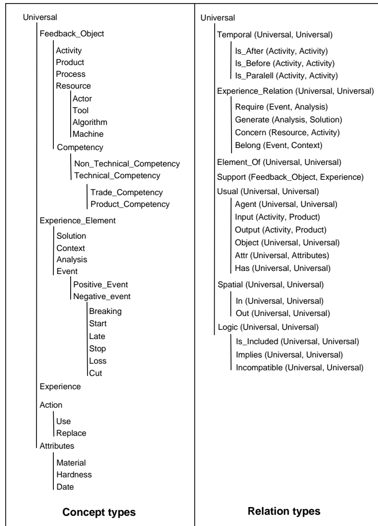
Figure 6. Formal ontology (lattice of concept and relation types) in conceptual graph
