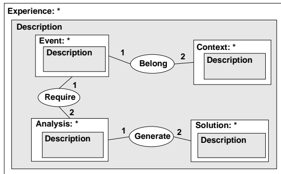
Figure 7. Generic experience GC
