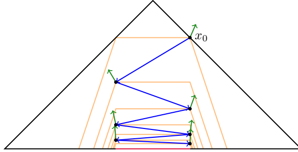
Figure 2: The constraint set (in black), polygonal sketches of the objective function (in orange), the solution set (in red), gradient directions (in green), and the trajectory (in blue) of the sequence (x_t)_{t \in \mathbb{N}} generated by the Frank-Wolfe algorithm with the line-search strategy (iii) starting from x_0 . The abscissa of x_t is (-1)^t/4 for all t \in \mathbb{N} , so (x_t)_{t \in \mathbb{N}} does not converge.
