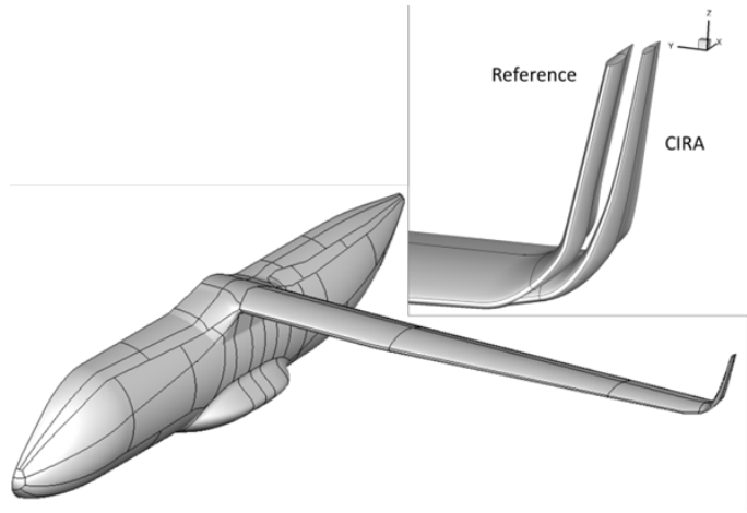
Fig. 13. Comparison of reference and CIRA winglet aeroshapes [15].
