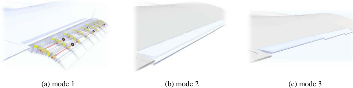
Fig. 6. Morphing Flap modes: (a) high-lift; (b) high speed tab; (c) high speed twist [25].
