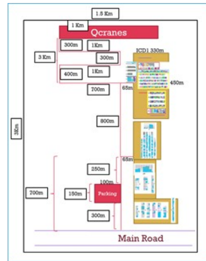
Figure 7: Draft of port layout for the simulation
