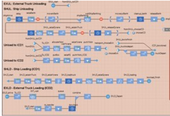
Figure 8: Event-based simulation flow of containers in the port operation
