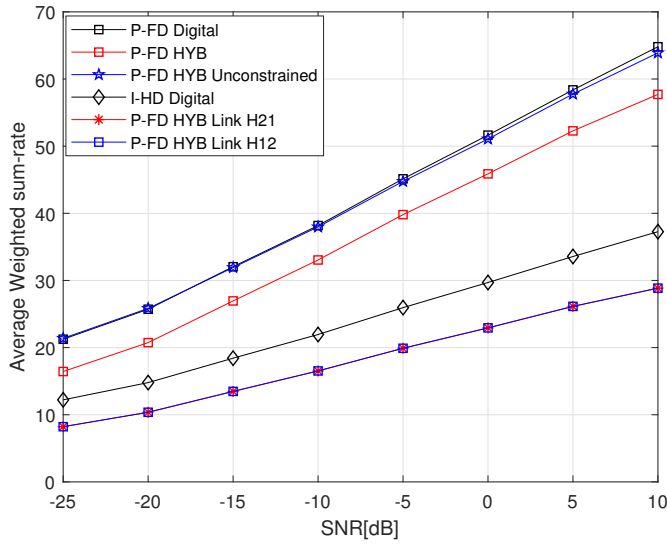
Fig. 2: Average WSR of a BD-FD system as function of SNR with k = \beta = -60 dB, with N_1 = N_2 = 100 , N_1^T = N_2^T = 32 and M_1 = M_2 = 20 .
