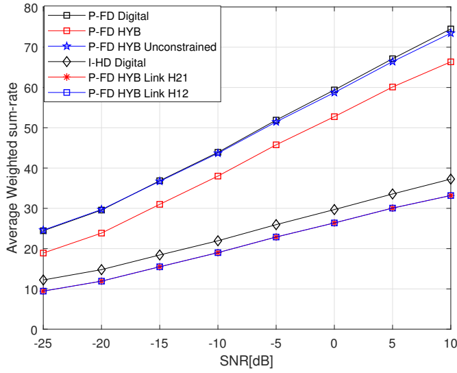
Fig. 1: Average WSR of a BD-FD system as function of SNR with k = \beta = -110 dB, with N_1 = N_2 = 100 , N_1^T = N_2^T = 32 and M_1 = M_2 = 20 .
