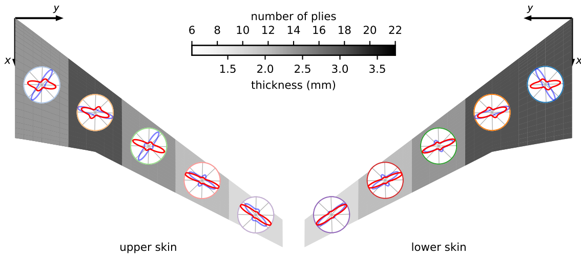
Figure 5 – Design point. The design variables – thickness and composite properties – are reported; the material properties are represented via the polar-plot of the engineering modulus, in red for the membrane-stiffness ( A tensor) and in blue for the flexion one ( D tensor).
