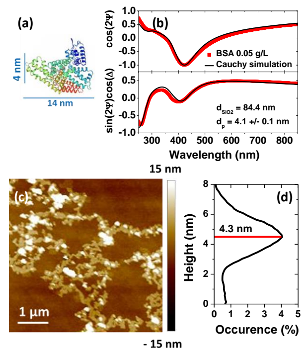
Fig. 2. Adsorption of BSA (from solution with concentration of 0.05 g/L) on SiO 2 surfaces: (a) representation of the 3D-structure of BSA, (b) Ellipsometric spectra of the adsorbed BSA, (c) PF-QNM AFM image of the protein organization and (d) height histogram of the adsorbed BSA.
