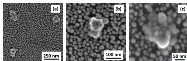
Fig. 5. SEM images showing deposition of BSA from a solution with concentration of 0.05 g/L on AgNPs.
