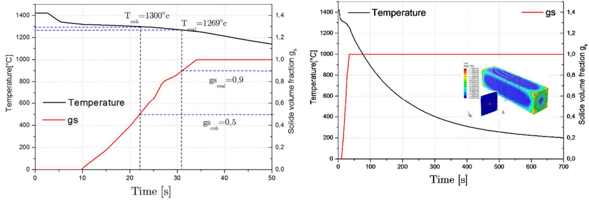
Figure 19. Evolution of temperature and solid volume fraction vs time in the center of the bar a) zoom of the time interval t \in [0s-50s] , b) plot of the time interval t \in [0s-700s]
