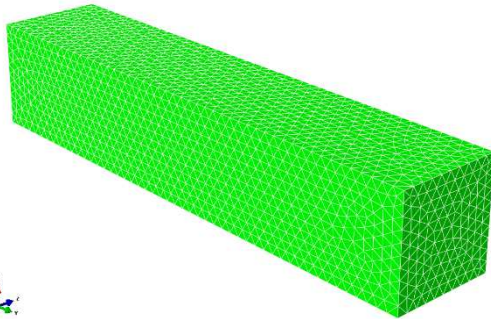
(c) Coarse mesh 51 000 elements
