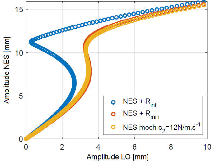
Figure 10: Slow Invariant Manifold of different NES configurations
