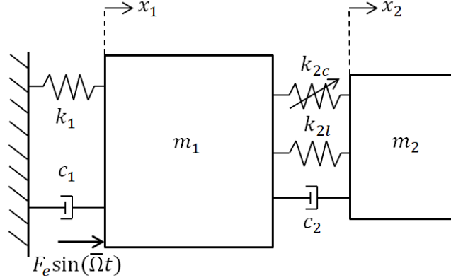
Figure 3: A linear principal oscillator coupled to an NES
