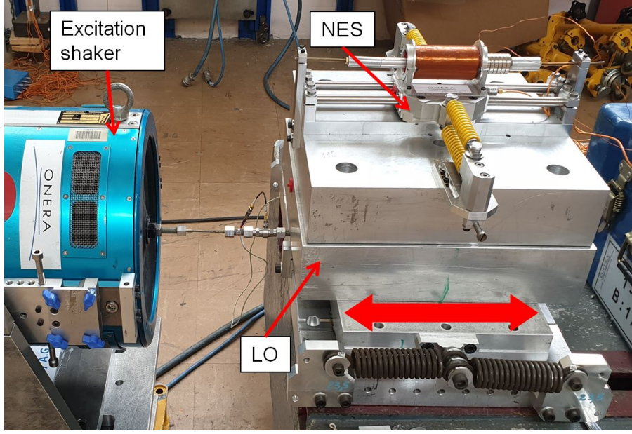
Figure 1: Prototype of the absorber with the magnet-coil system
