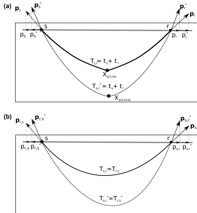
Figure 2. Slopes serving as a objective measure in slope tomography. (a) In the case of reflection slope tomography: the two-way traveltimes T_{s,r} (simulated through the computed one way traveltimes t_s and t_r ) and the slopes at the source and receiver positions, p_s and p_r are needed to constrain the velocity model and the scattering point position X_{sct} . (b) In the case of FASTT: the slopes at the source and receiver positions, p_{r,s} and p_{s,r} supplement the two-way traveltimes T_{s,r} during the velocity model inversion by constraining implicitly the geometry of the ray. The star and the square denote the source and receiver positions (with their respective slowness vectors). The recorded data are labelled with the superscript *. The dash line represents the true rays.T
