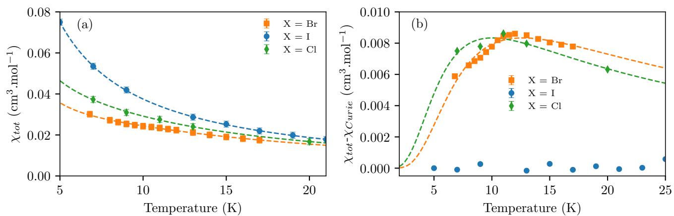
Figure S6. (a) Temperature dependence of the spin susceptibility in the low-temperature region for (o\text{-DMTTF})_2\text{Br} , X = Cl, Br and I. The dashed lines are the best fit using eq.(6). (b) Difference between the susceptibility \chi_{tot} and the Curie law component in eq.(6). The dashed lines are the best fit of \chi_{tot} using eq.(6) without the Curie law component.
