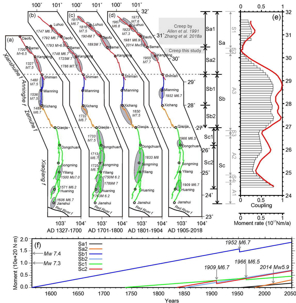
Figure 6. (a–d) Maps for four historical periods of damaged areas for 36 M \geq 6 earthquakes along the XXFS (modified from Wen, Ma, et al., 2008). Gray ellipses show the damaged areas for every earthquake together with the earthquake date and magnitude proposed by Wen, Ma, et al. (2008). The red, blue, yellow and green lines correspond to the Xianshuihe fault, the Anninghe fault, the Zemuhe fault and the Xiaojiang fault respectively. (e) The red line corresponds to the vertically averaged coupling coefficients above 10 km depth. Gray histograms represent cumulative seismic moments every 0.2° bin between 0 and 20 km depth. (f) Moment deficit accumulation and released through earthquake as a function of time since 1536, for the 6 segments of the XXFS labeled in (a–d).
