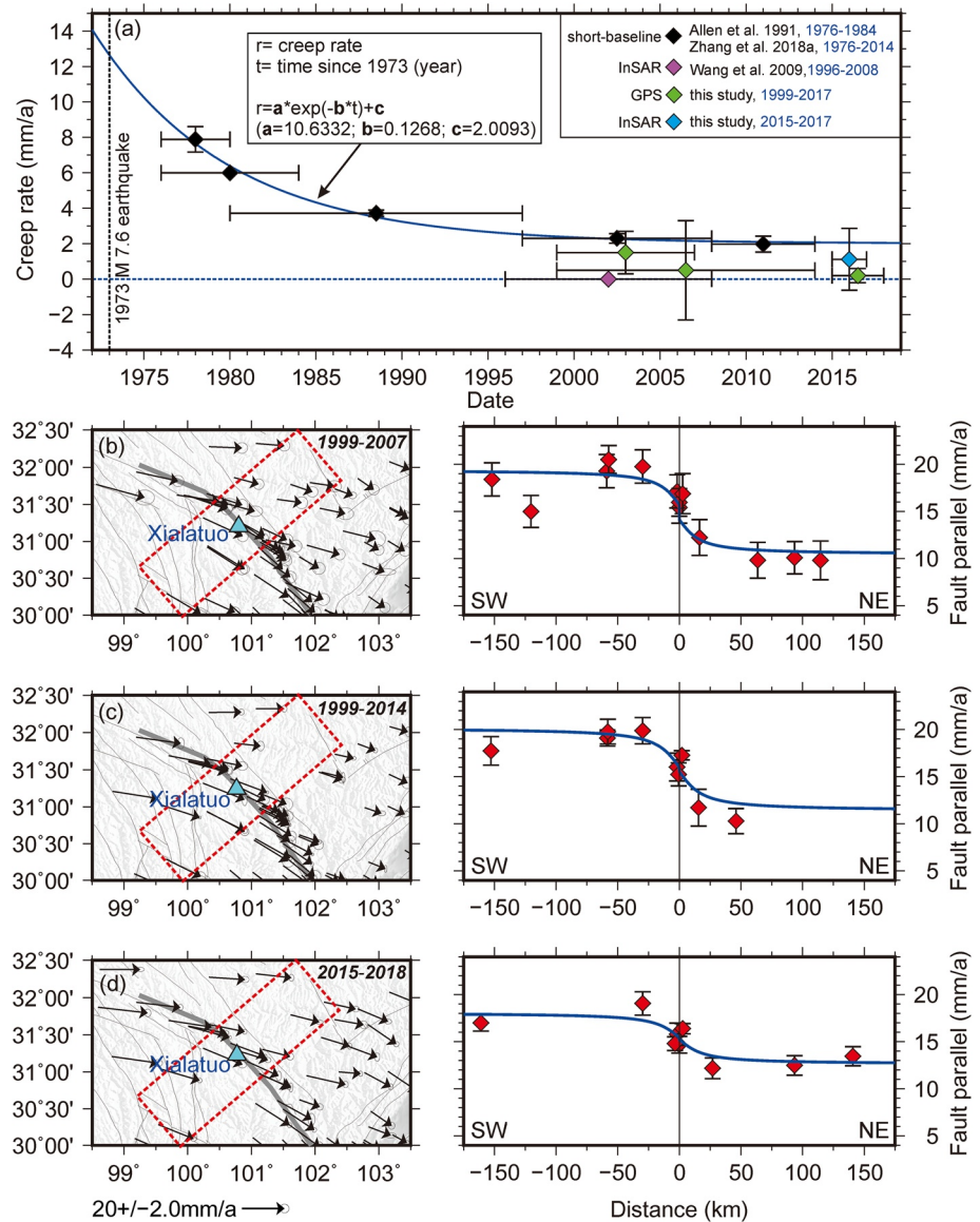
Figure 8. (a) Fault creep rate at the Xialatuo site as a function of time. Blue solid line is the best decreasing exponential fit of short-baseline measurements. Vertical error bars show 1- \sigma uncertainty, horizontal error bars show the time period used for each measurement. (b) GPS velocity solution (Eurasia fixed reference frame, error ellipses at 68% confidence levels) in 1999–2007 and corresponding fault parallel velocities across the Xialatuo site (error bars show 1- \sigma uncertainty), with its locations shown in red rectangles in the left panel. Blue solid line represents the best fitting curve. (c) and (d) are GPS velocity solutions (Eurasia fixed reference frame) for the 1999–2014 and 2015–2018 periods respectively. Fault normal components are shown in Figure S12 in Supporting Information S1, and PDFs of estimated fault parameters are shown in Figure S13 in Supporting Information S1.
