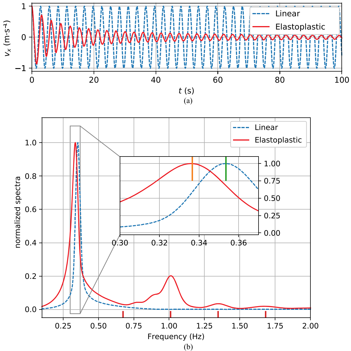
Figure 6. (a) Time evolution of the X-component of velocity at point (1.0,1.0,0.5) for linear and elastoplastic media ( \gamma_{\text{ref}} = 5 ). (b) Normalized Fourier spectra of the previous traces. The colour version of this figure is available only in the electronic edition.
