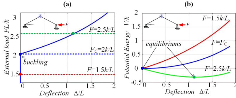
Fig. 2 Straight initial configuration: the force-deflection and energy curves for two-link mechanism (case \alpha=0 ).
