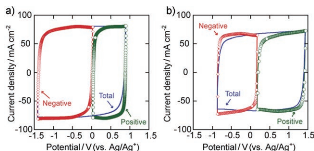
Figure 2. Cyclic voltammograms (CVs) taken at a scan rate of 20 \text{ mVs}^{-1} on samples synthesized at a) 500 and b) 800 °C. The plot of total current density versus potential represents the response of both the positive and negative electrodes as the potential is scanned. The positive- and negative-electrode responses are separated from one another by using a third silver quasi-reference electrode placed between the electrodes. As the current in the cell is limited by the lower-capacitance electrode, the different sizes of the voltage windows in a CV plot are indicative of different capacitance values at the positive and negative electrodes. This is most clearly reflected in the TiC-CDC sample synthesized at 500 °C.
